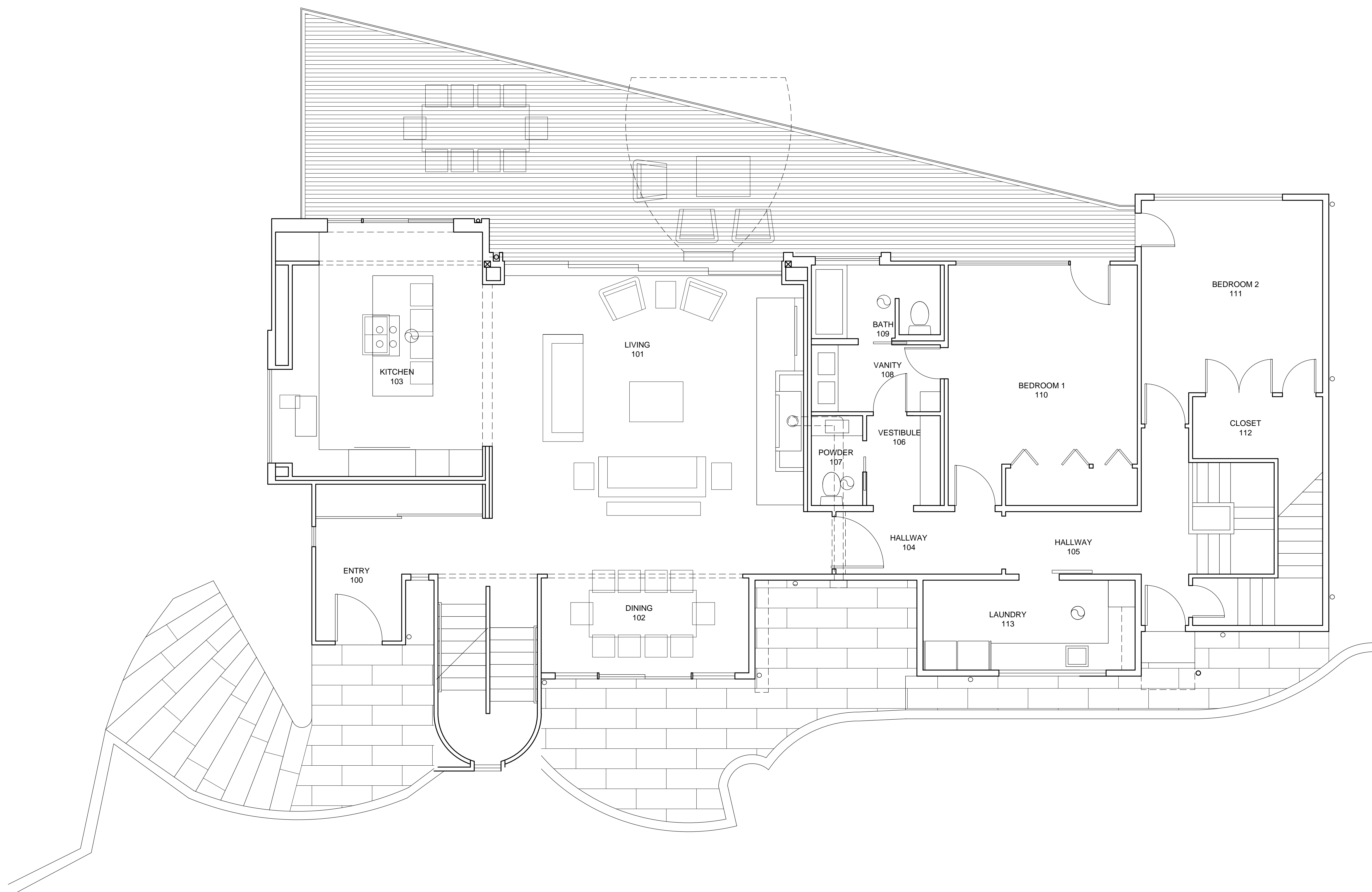
1 FIRST FLOOR PLAN
